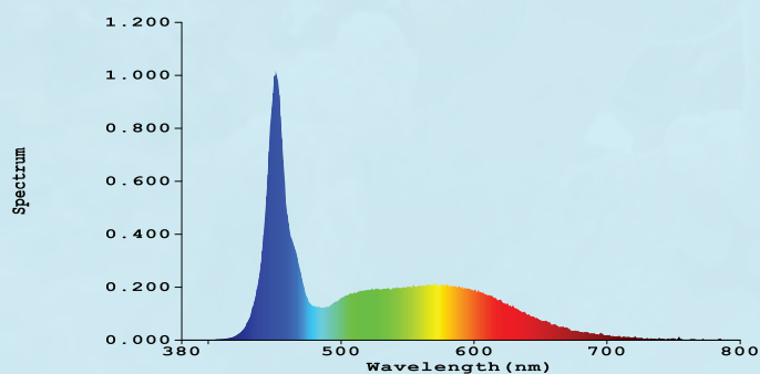
Spectrograms
